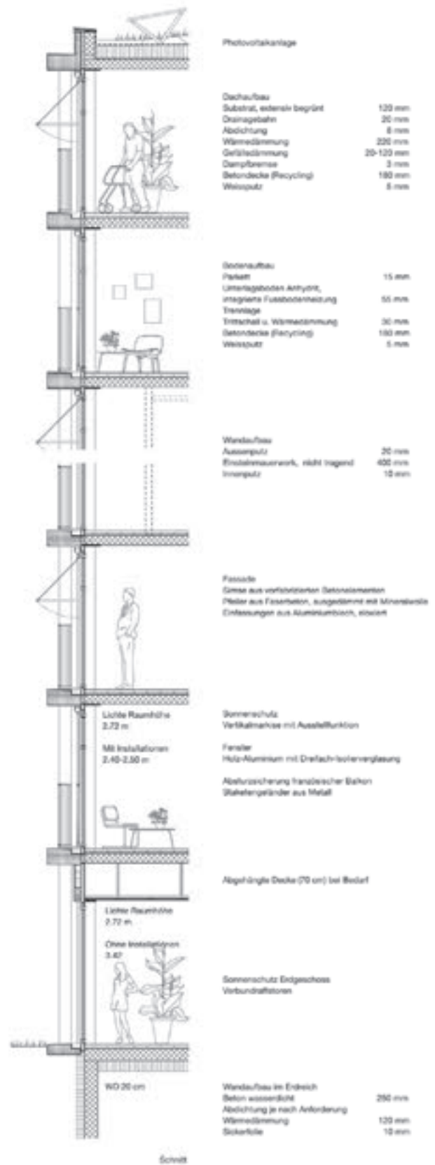
Detail 1:100
