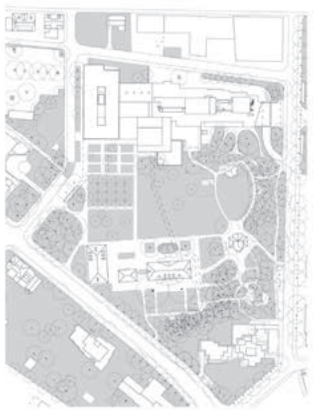
Situation 1:2750
