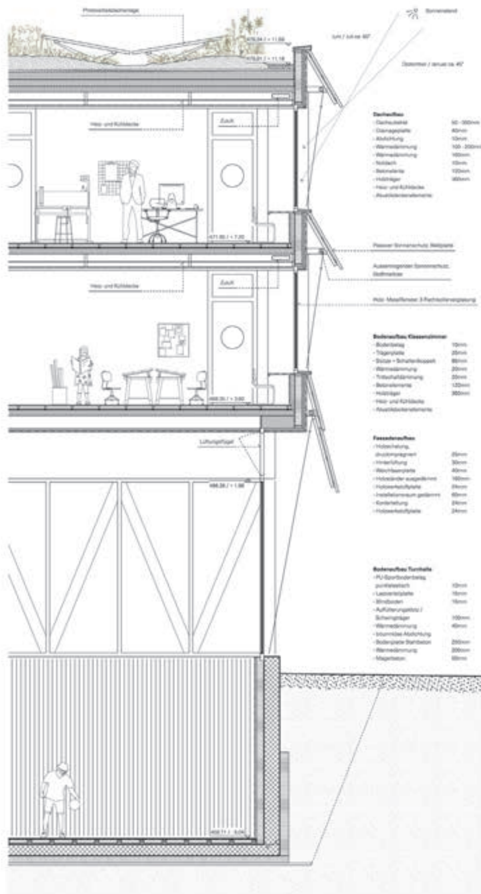
Detail 1:85
